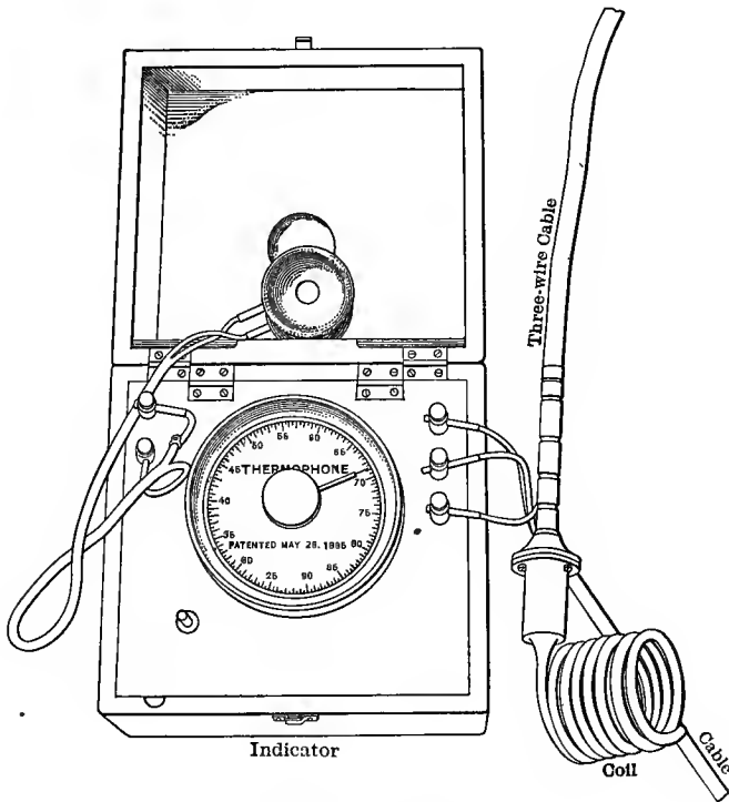
FIG. 36.—Thermophone.
