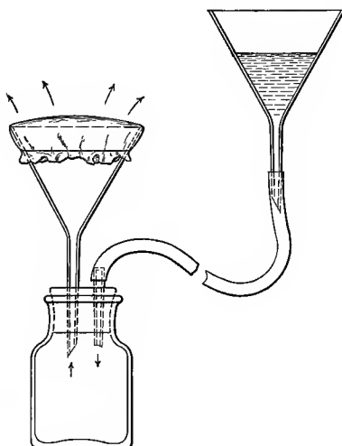
FIG. 7.—Apparatus for Concentrating Microscopic Organisms.
