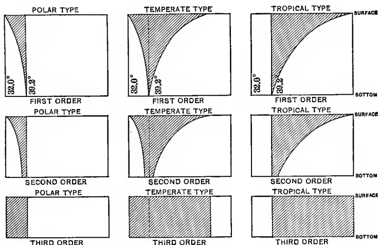
FIG. 43.—Classification of Lakes According to Temperature.
