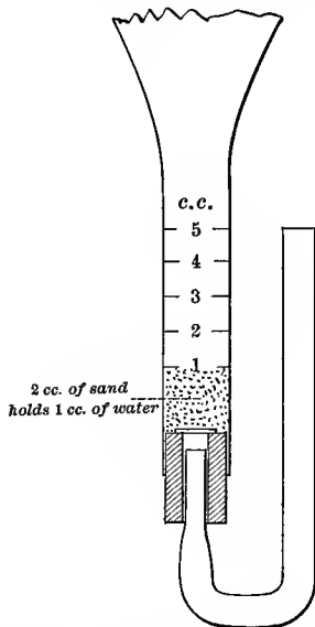
FIG. 15.—Concentrating Attachment.
