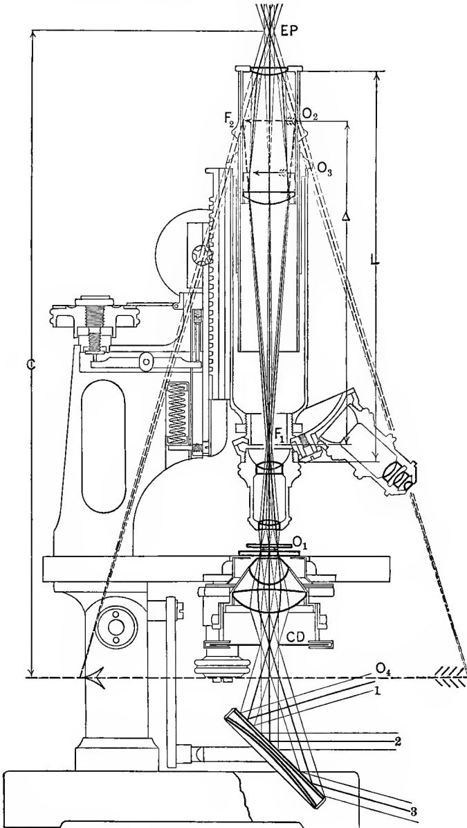
FIG. 23.—Optics of the Compound Microscope. After Bausch.
