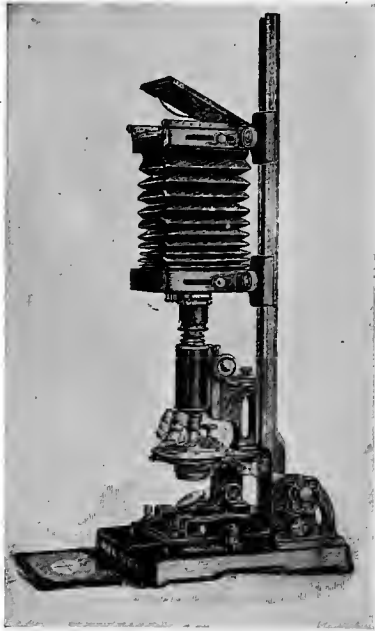
FIG. 29.—Photomicrographic Camera.
