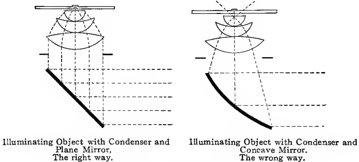
FIG. 26.—Illumination with Plane and Concave Mirrors.
