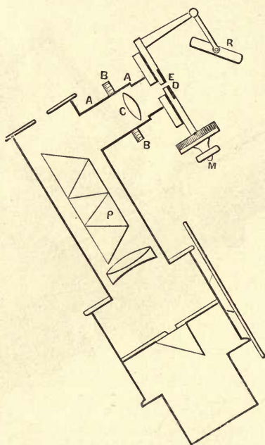
Spectroscope with Micrometer.
