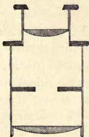
Huygenian Eye-piece.
