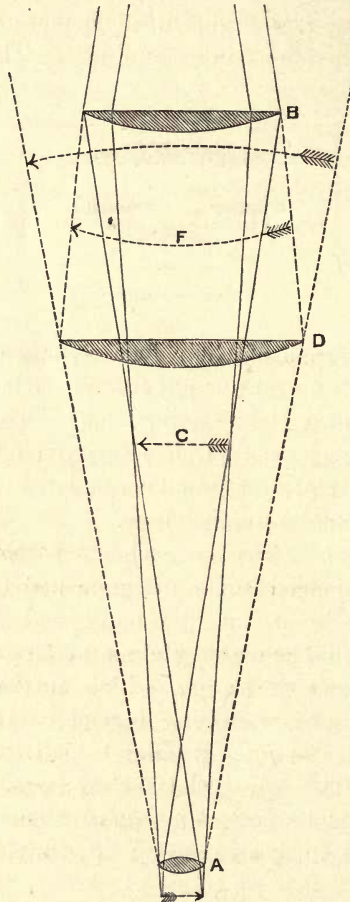
Compound Microscope.
