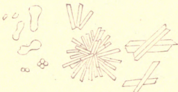
Phosphate of Lime.
