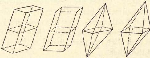
Principal Axes.
