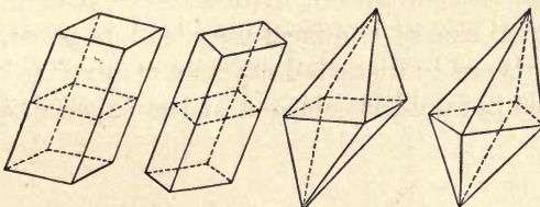
Principal Axes.
