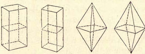
Principal Axes.
