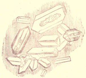
Ammonio-phosphate of Magnesia.
