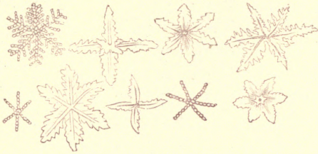
Ammonio-phosphate of Magnesia.
