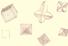
Chloride of Sodium.
