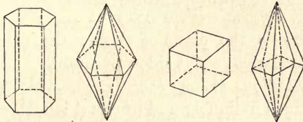
Principal Axes.
