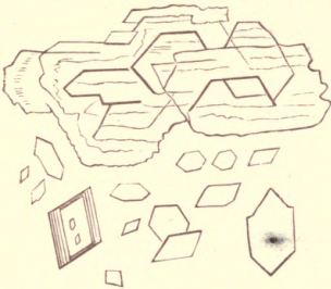
Nitrate of Urea.
