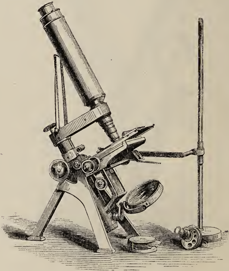
Fig. 38.— Powell and Lealand's Microscope, with Amici prism, arranged for the oblique illumination of test-objects.
