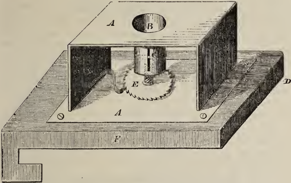
Fig. 66.—Section Cutting Machine.
