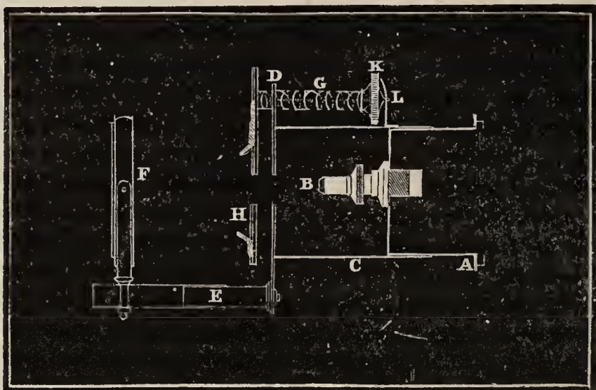
Fig. 99.—Highley's Camera.
