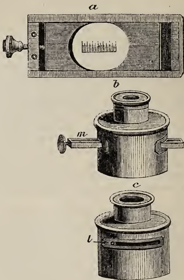
Fig. 35.—Mr. Jackson's Micrometer eye-piece.
