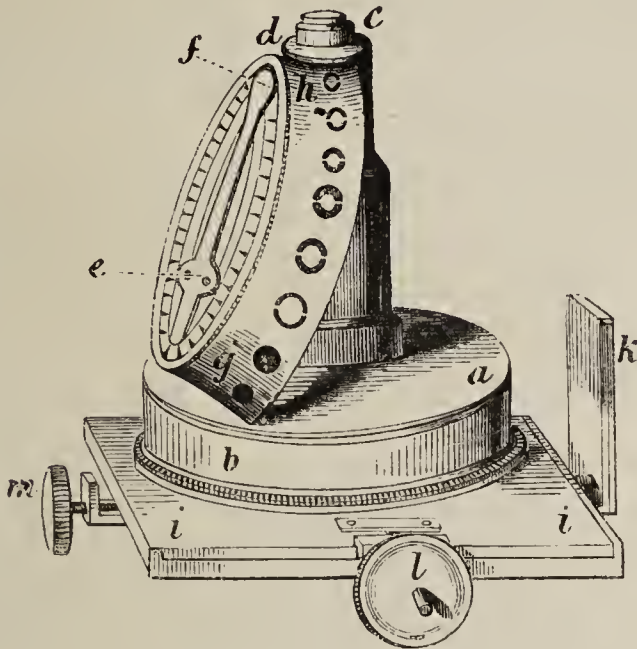
Fig. 42.— Gillett's Condenser.
