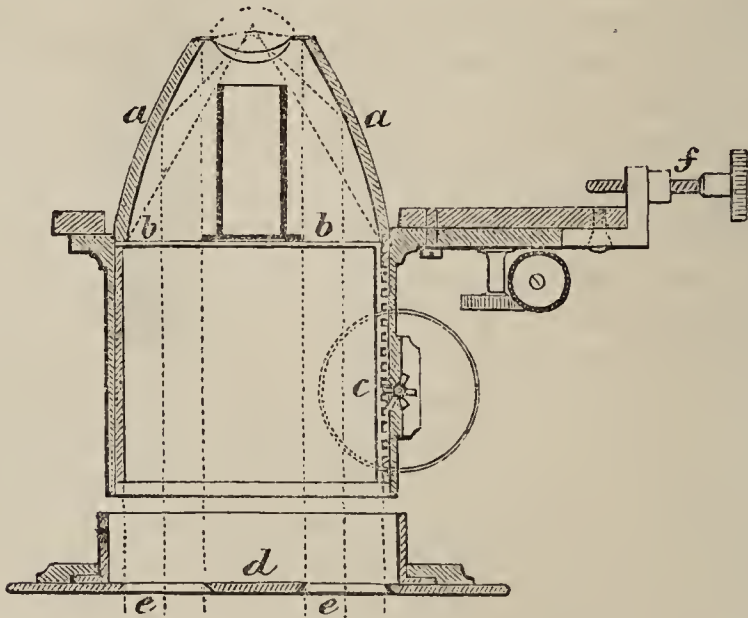
Fig. 44.—Wenham's Parabolic Reflector.
