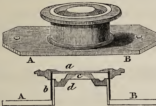
Fig. 57.—Varley's Animalcule-cage.
