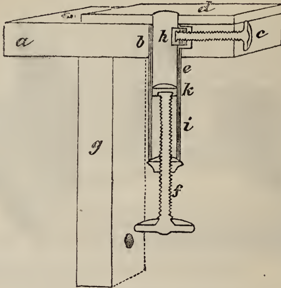
Fig. 67.— Topping's Section Cutting Machine.
