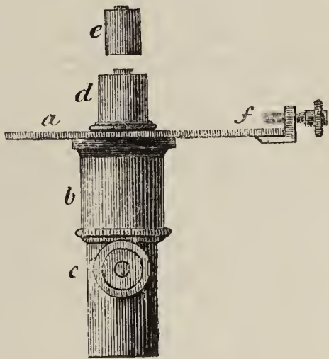
Fig. 43.—Ross's Condenser.
