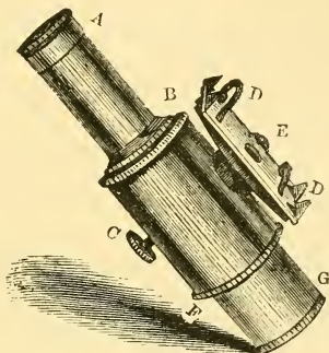
Fig. 75.— The Sorby-Browning Micro-spectroscope.
