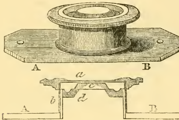
Fig. 121.—Varley's Animalcule-cage.
