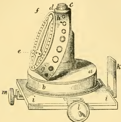
Fig. 99.—Gillett's Condenser.
