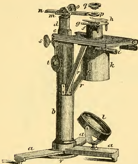
Fig. 24.— Valentine's Microscope.
