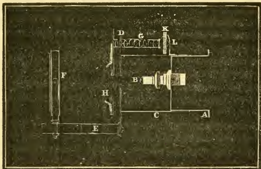
Fig. 96.—Highley's Camera.
