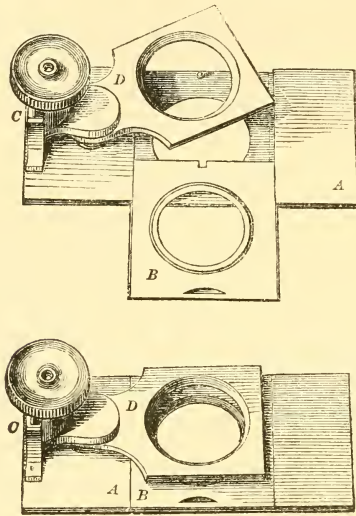
Fig. 122.—Ross's Compressorium.
