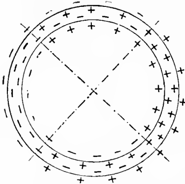
Distribution of Electricity upon the Plates.
