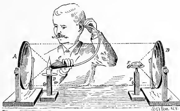
Reflection of Light and Sound.
