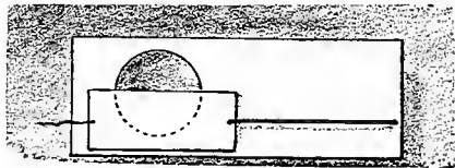
Slide showing the Tiring of the Eye.
