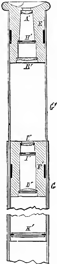
Terrestrial Eyepiece
