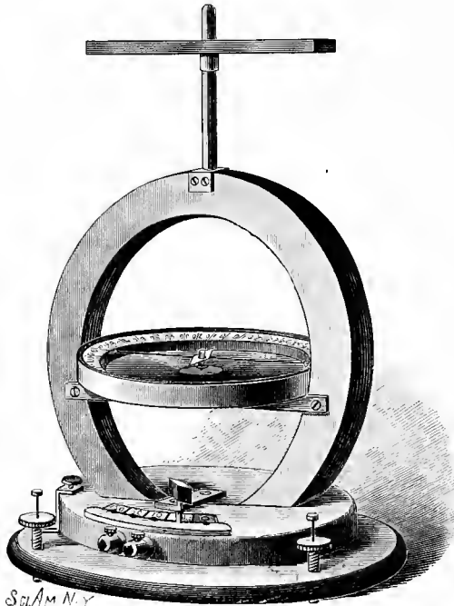
Tangent Galvanometer.
