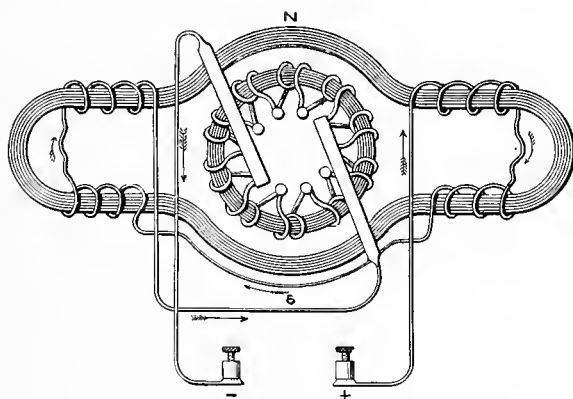
Circuit of Simple Electric Motor.
