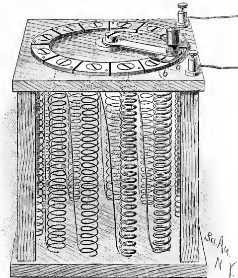
German Silver Rheostat.
