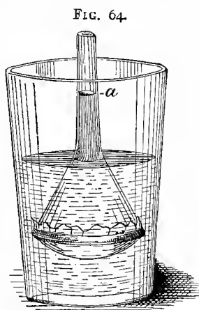
Endosmometer.
