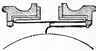
Speaking Diaphragm.
