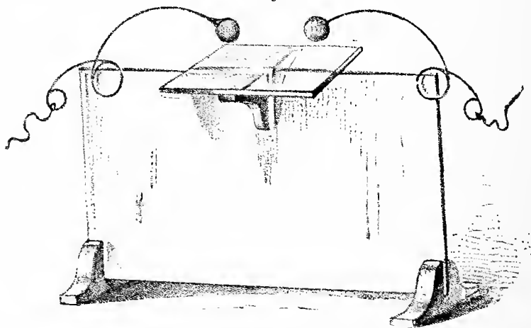
Universal Discharger.
