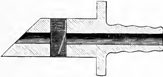
Valve for Compression Pump.
