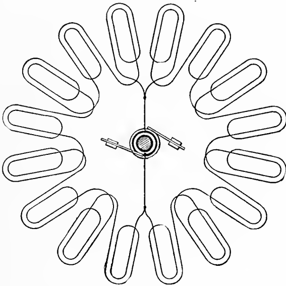
Diagram of Armature Coils and Connections.
