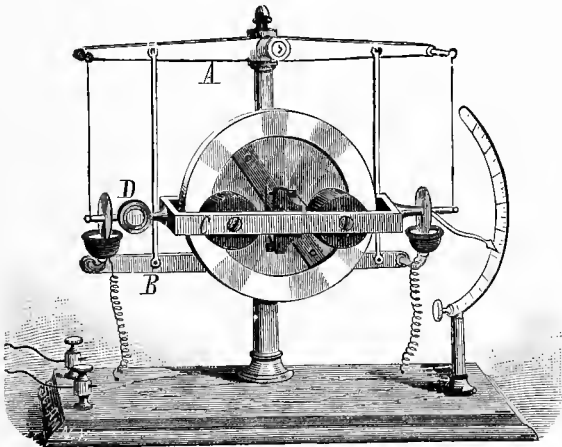
Electrical Indicator.
