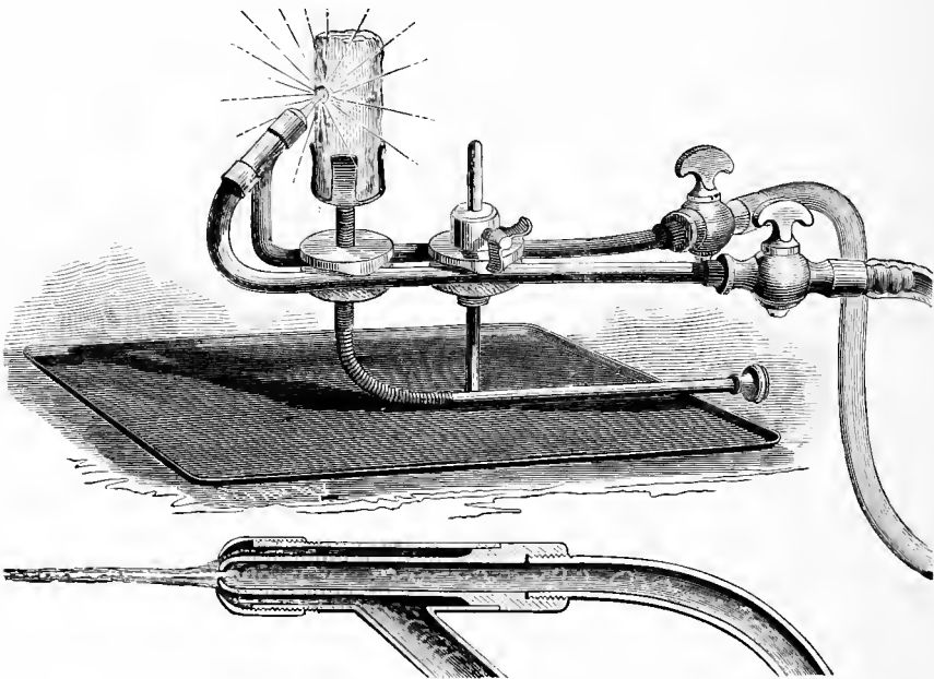
Annular Oxyhydrogen Burner.
