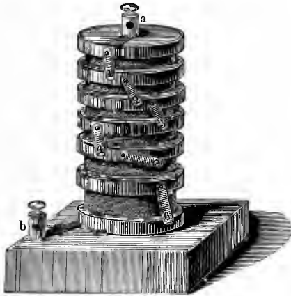
Resistance Column
