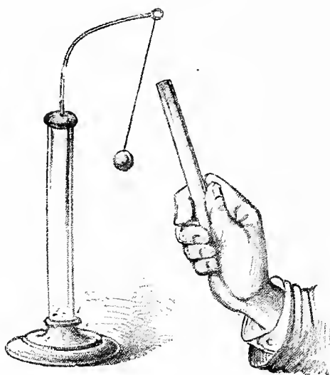
Electric Pendulum.
