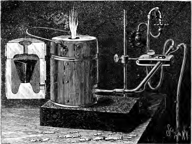
Blowpipe Furnace.
