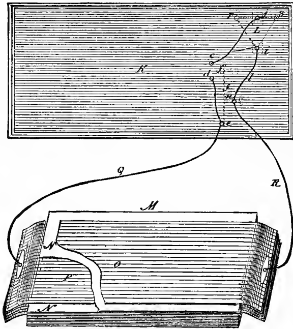
Diagram of Condenser Connections.
