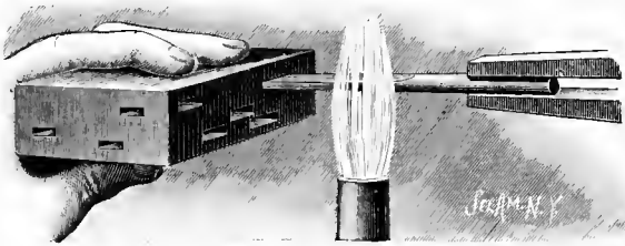
Softening the Shank of a Drill.
