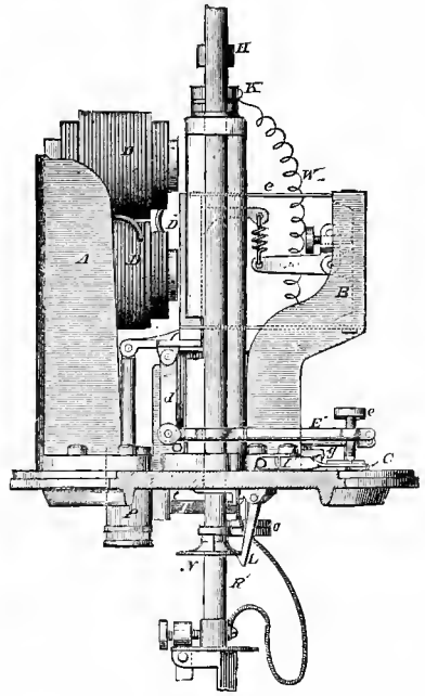
Feeding Mechanism of the Weston Arc Lamp.
