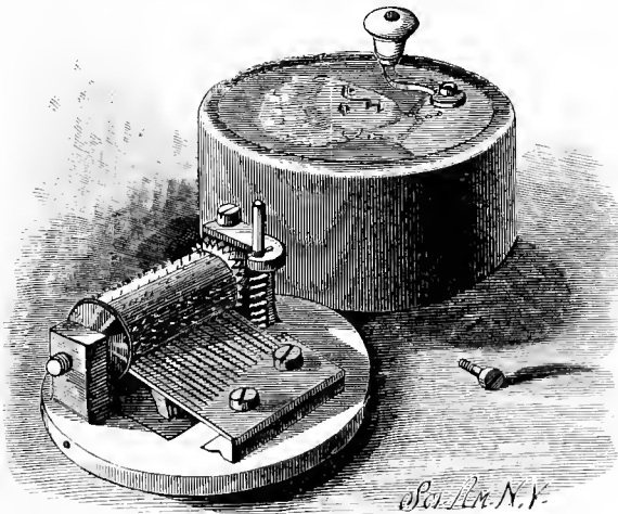
Music Box
