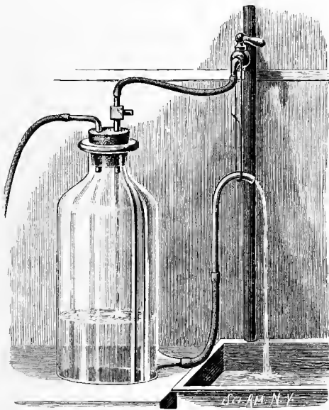
Blast produced by the Aspirator.
