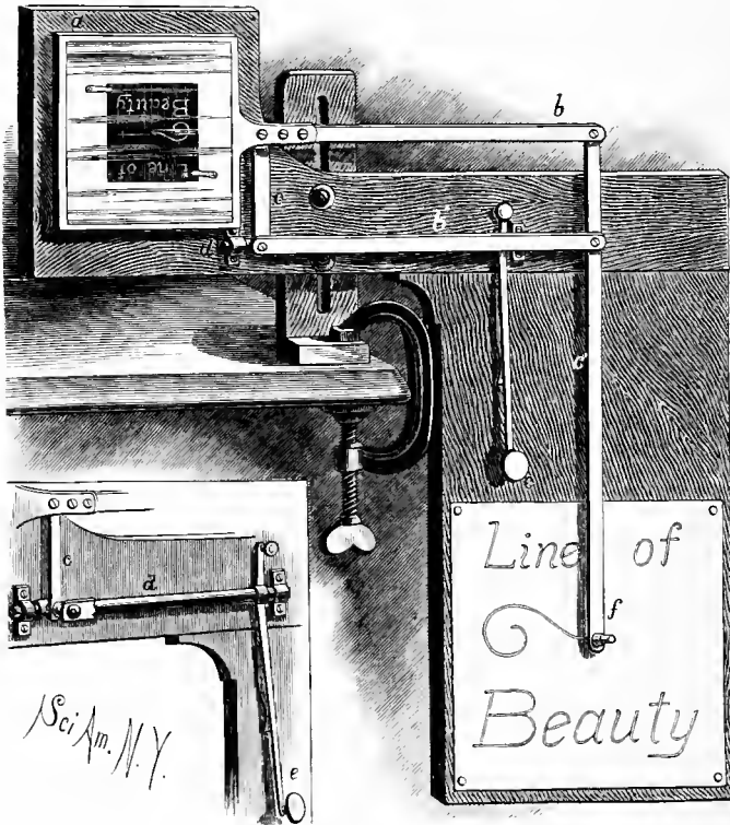
Lantern Pantograph.
