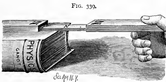
Consequent Pole.
