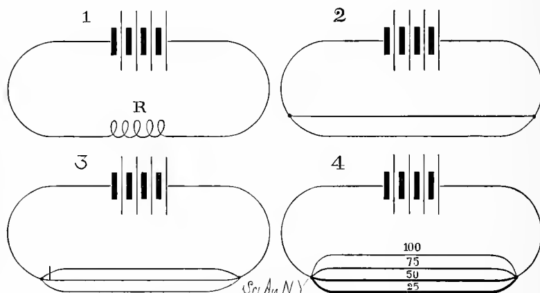
Branch Circuits.
