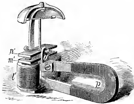
Simple Polarized Bell.
