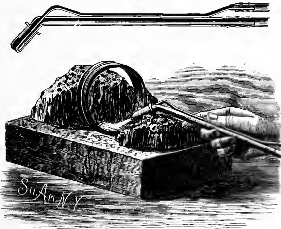
Brazing.
