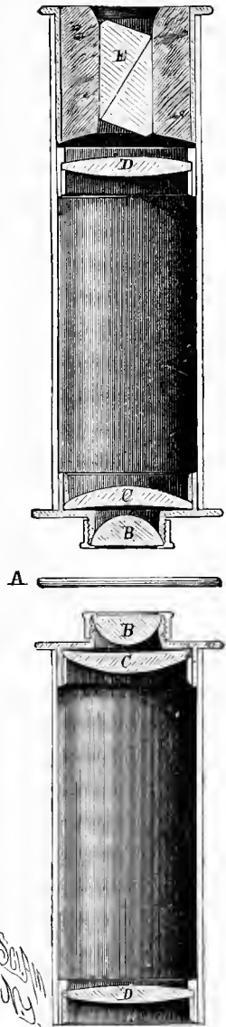
Longitudinal Section of Tubes of Polariscope.
