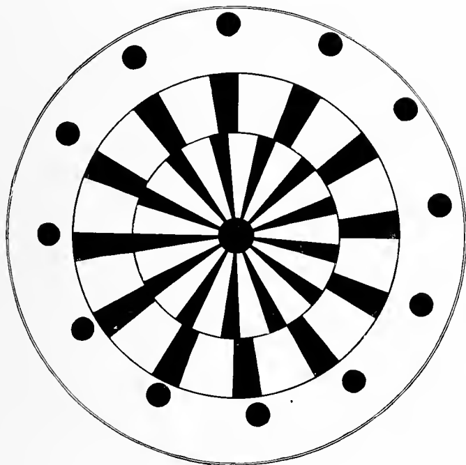
Rotary Disk.
