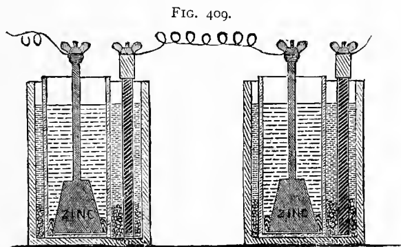
The Fuller Cell.
