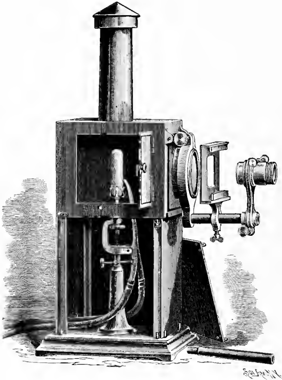
Scientific Lantern.
