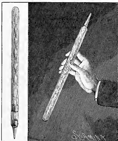
Self-exciting Geissler Tube.
