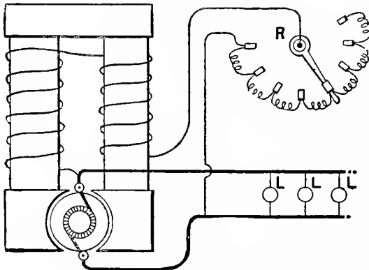
Edison's System of Regulating.
