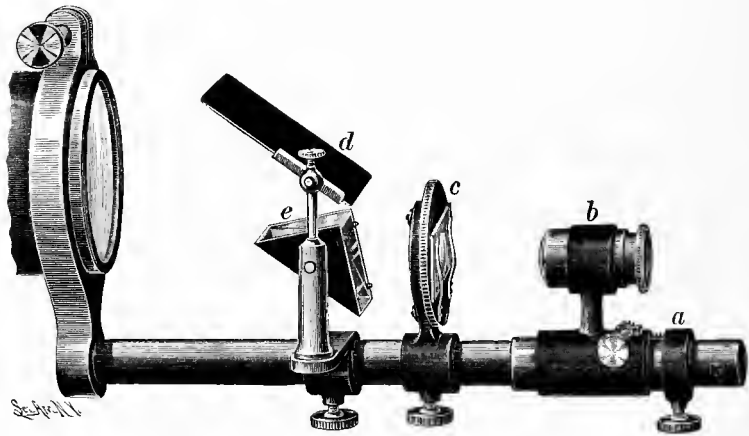
Lantern Polariscope.
