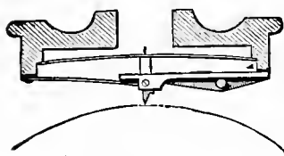
Receiving Diaphragm.
