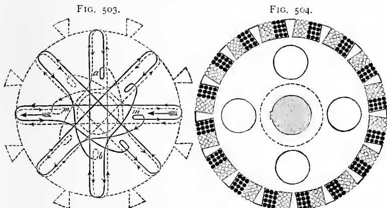
Diagram and Cross Section of Weston Armature.
