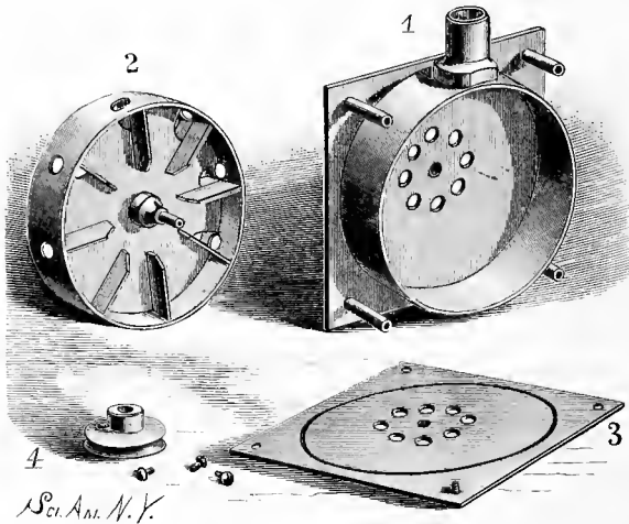
Details of the Siren.
