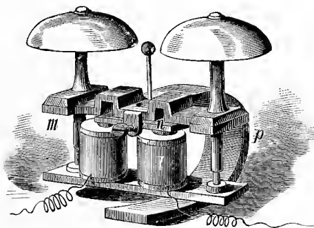
Polarized Bell.
