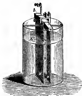
Smee's Battery.
