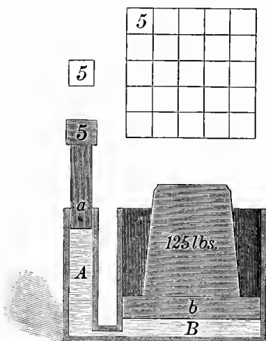
Principle of Hydraulic Press.
