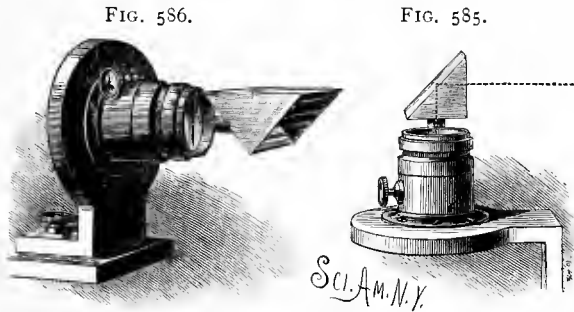
Application of the Ninety Degree Prism.
