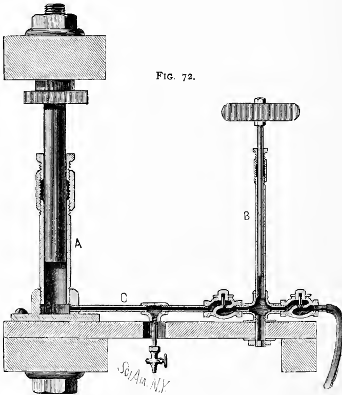
Sectional View of Simple Hydraulic Press.
