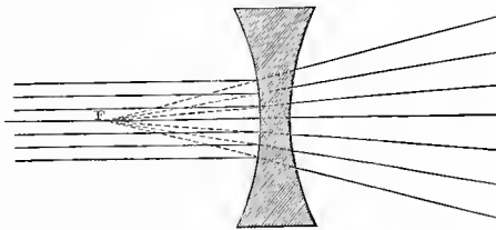
Principal Focus of a Concave Lens.
