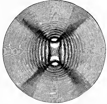
Niter.
