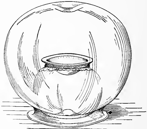
Partial Vacuum by Exosmose.
