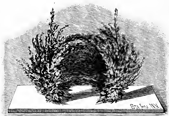
Arborescent Magnetic Figures.
