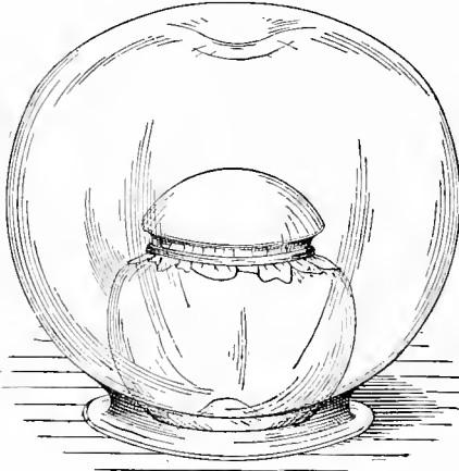
Pressure by Endosmose.
