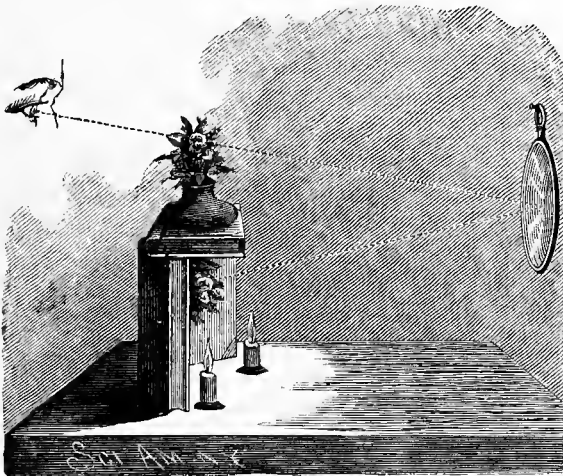
Concave Mirror, Phantom Bouquet.
