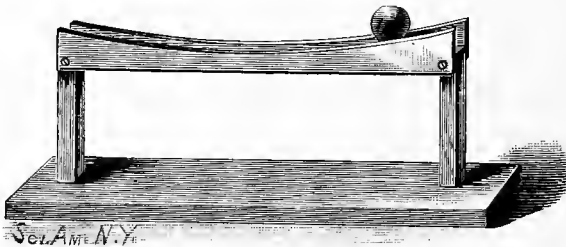
Cycloid Curve.
