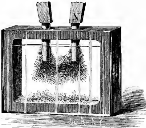
Magnetic Field.
