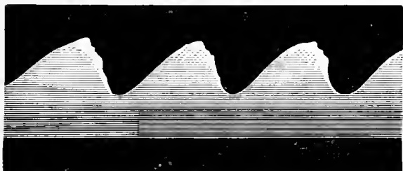
Waves.
