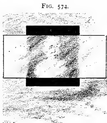
Refraction.
