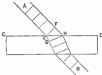
Refraction.
