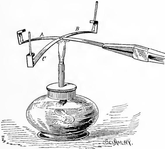
Conduction of Heat.
