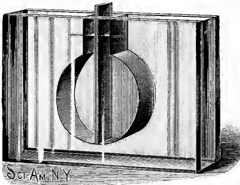
Reduction of Volume by Mixture.
