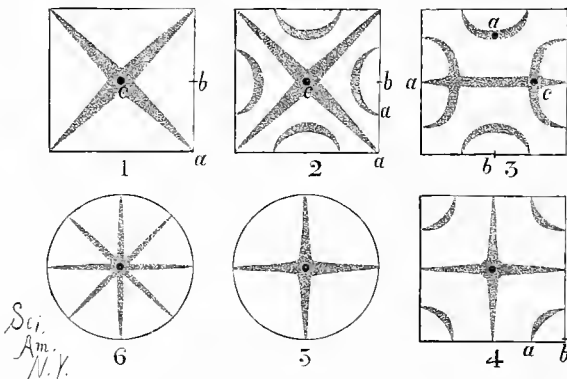
Sand Figures.
