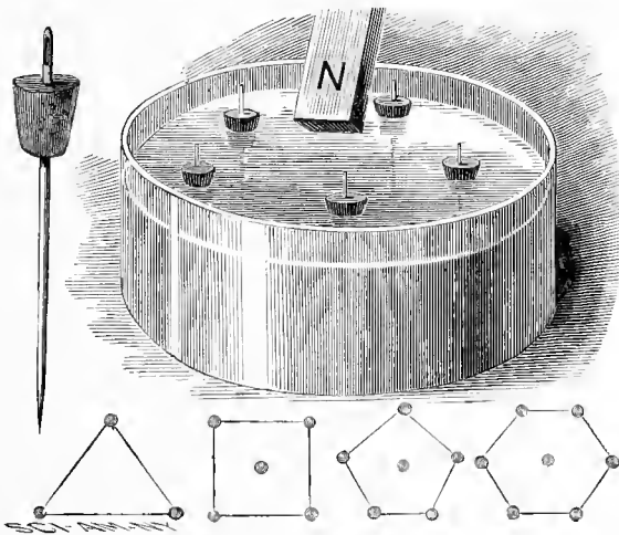
Mayer's Floating Needles.
