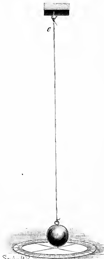
Foucault's Experiment.
