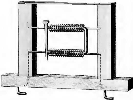
Sturgeon's Magnet.
