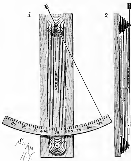
Metallic Thermometer.
