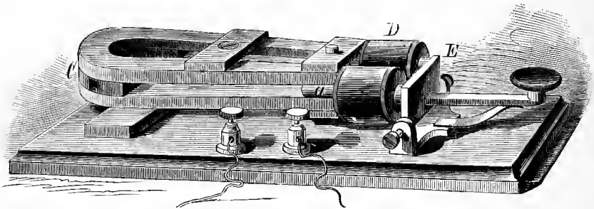
Magnetic Key.
