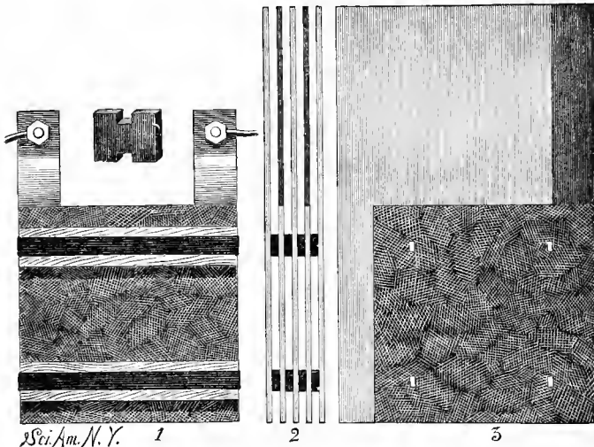
Plates of Secondary Battery.
