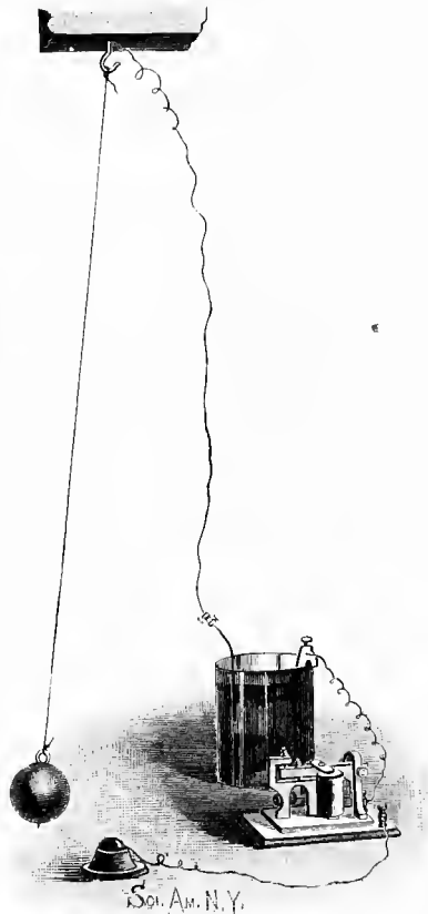
Pendulum with Audible Beats.
