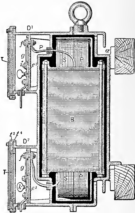
Section of Converter and Casing.
