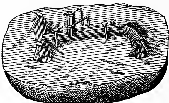
Method of holding Work for soldering.
