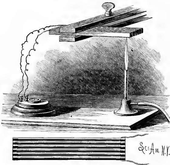
Thermo-Electric Series.
