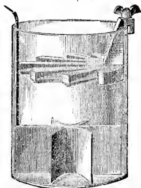
Gravity Battery.
