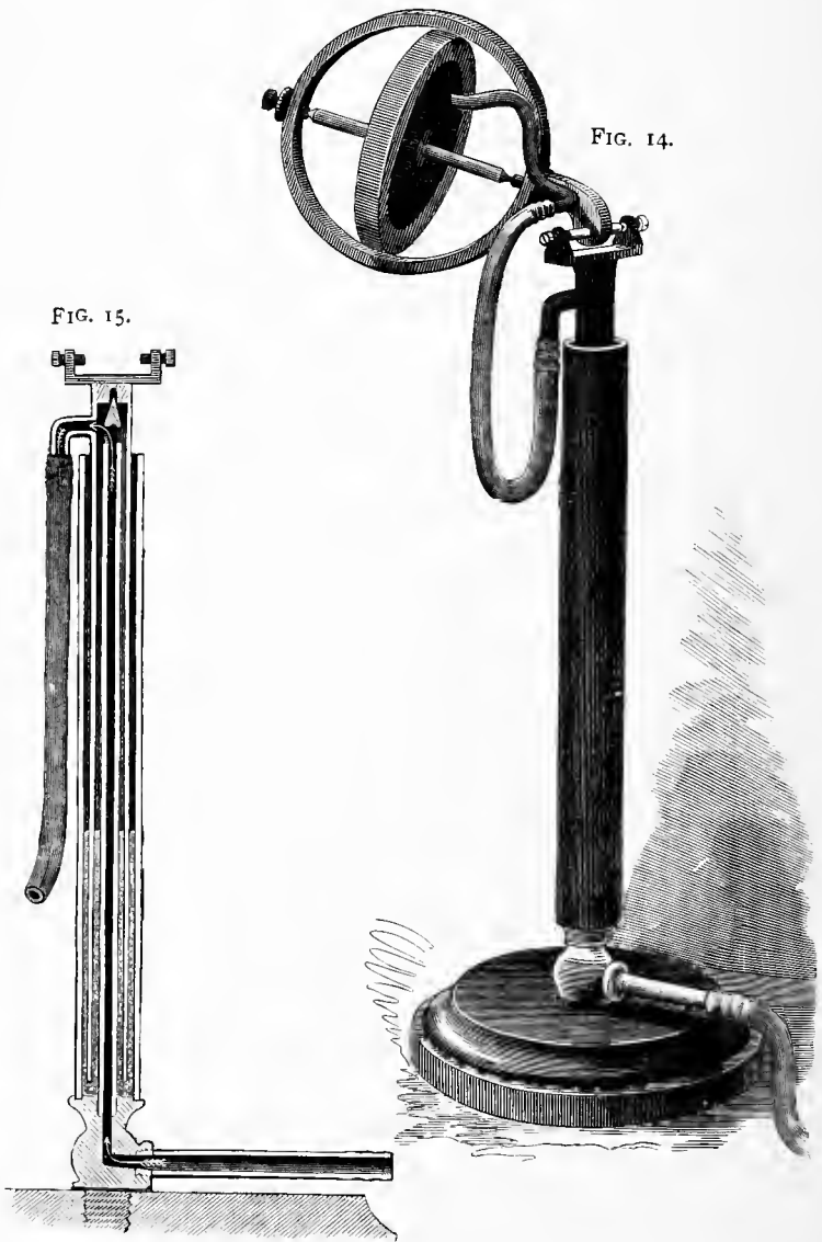
Pneumatic Gyroscope.
