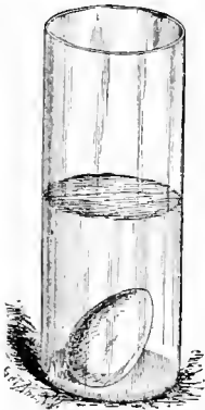
Egg in Fresh Water.
