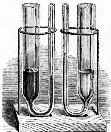
Capillary Elevation and Depression.
