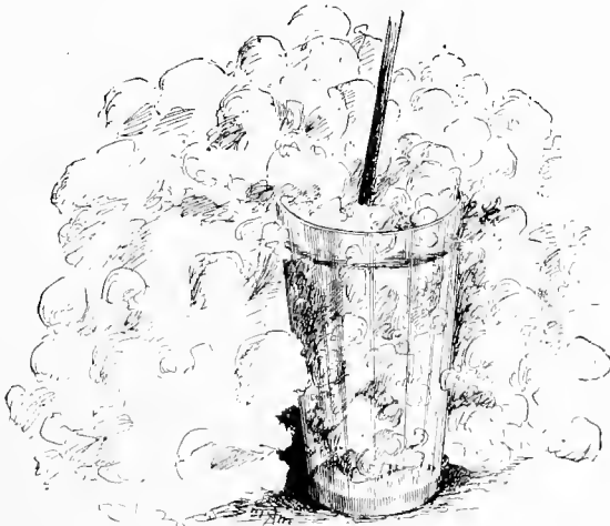
A Hatful of Cotton in a Tumblerful of Alcohol.
