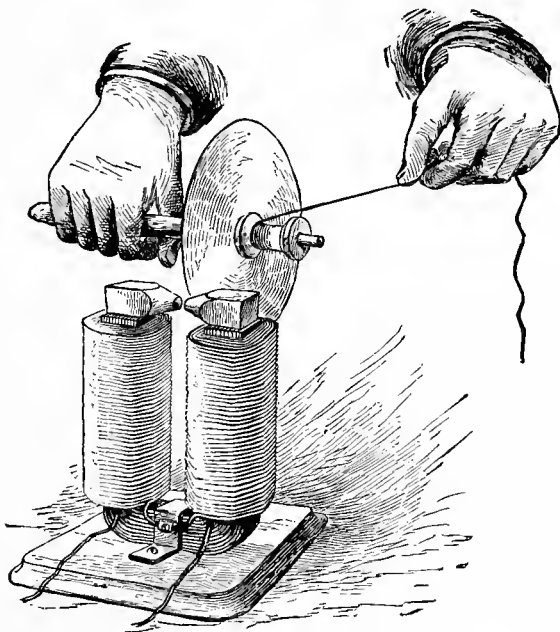
Foucault's Experiment.
