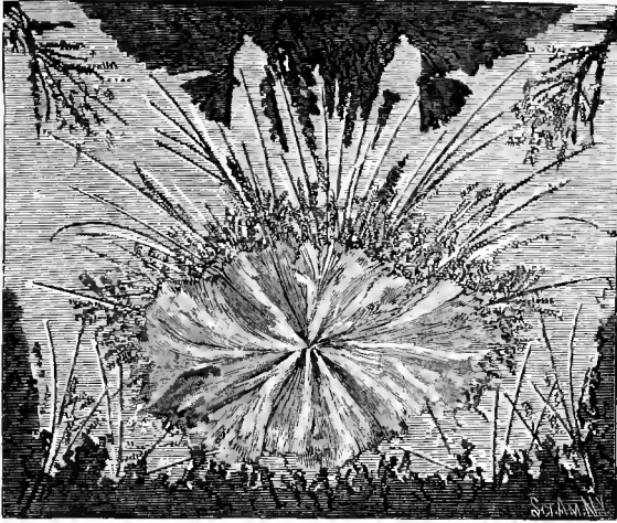
Santonine.
