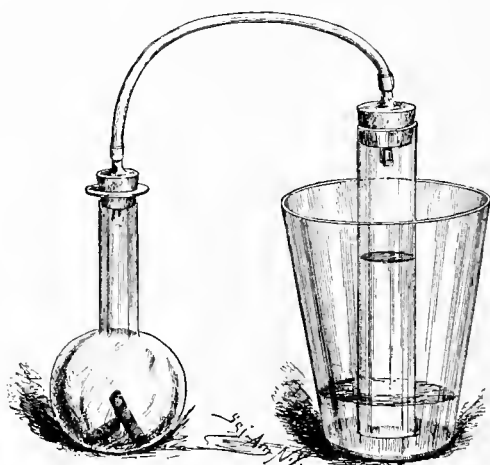
Absorption of Carbonic Acid Gas by Charcoal.
