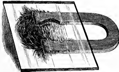
The Magnetic Field.
