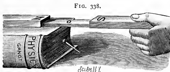
Neutral Point between Unlike Poles.
