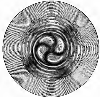
Airy's Spirals.
