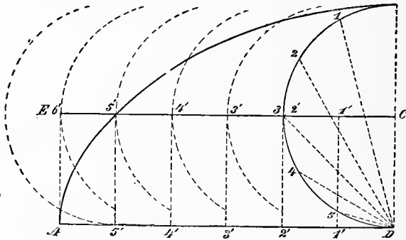
Method of Describing the Cycloid.
