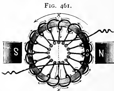
Armature in Magnetic Field.
