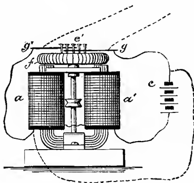
Gramme Machine for Illustration.
