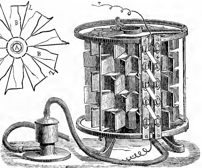
Clamond's Thermo-Electric Battery.
