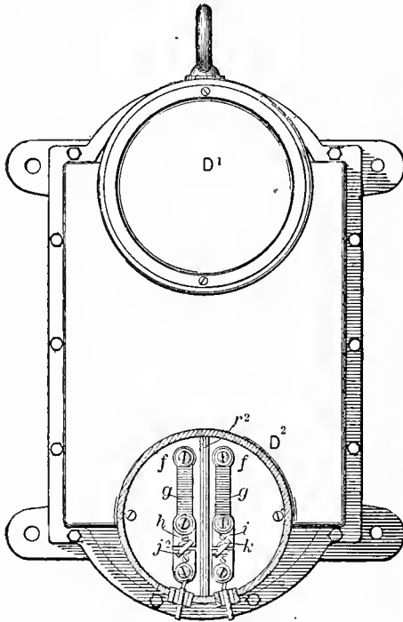
Front View of Converter.
