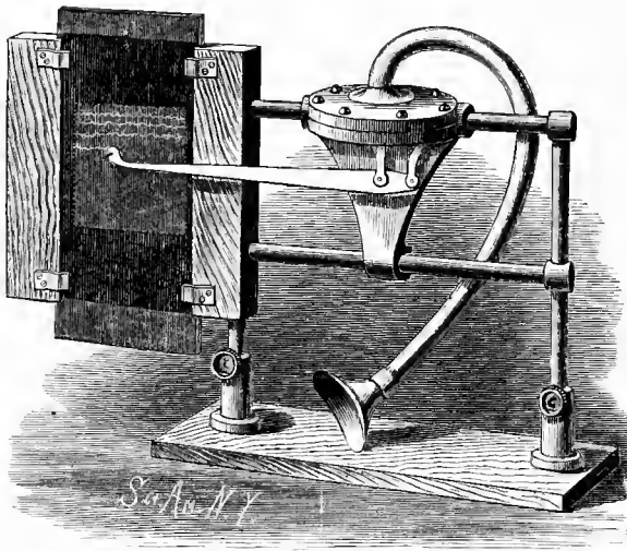
Phonographic Recorder.
