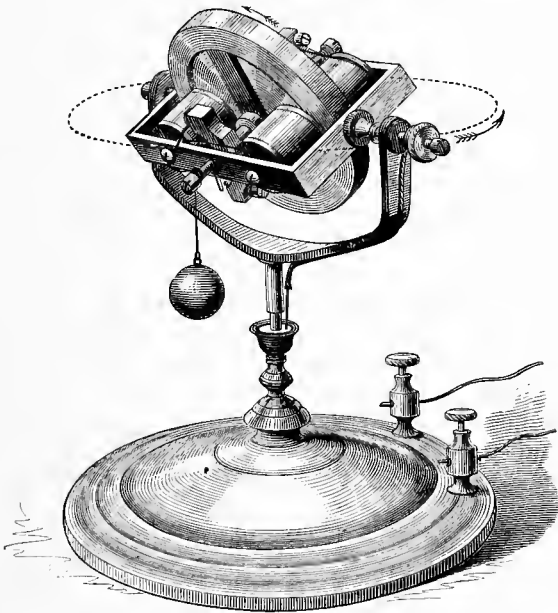
Electrical Gyroscope.
