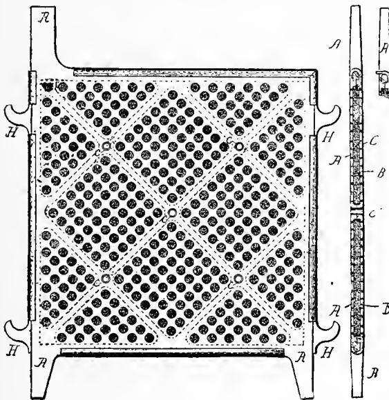
Plate of Storage Battery.
