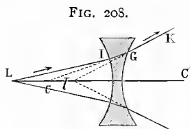
Diverging Rays, Concave Lens.
