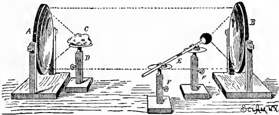
Reflection of Heat.
