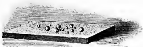
Surface Tension exhibited in Water Drops.
