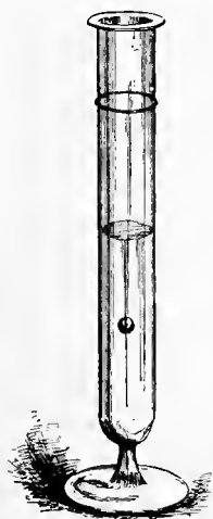
Oil Globule suspended in Equilibrium.
