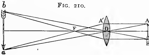
Real and Magnified Image.
