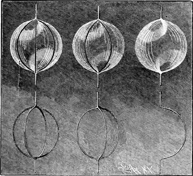
Rapiieff's Optical Illusion.
