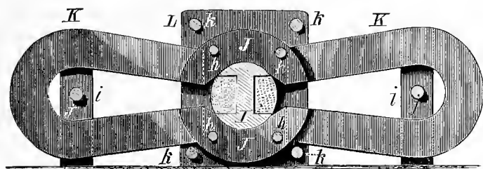
Transverse Section of Magneto-Electric Machine.
