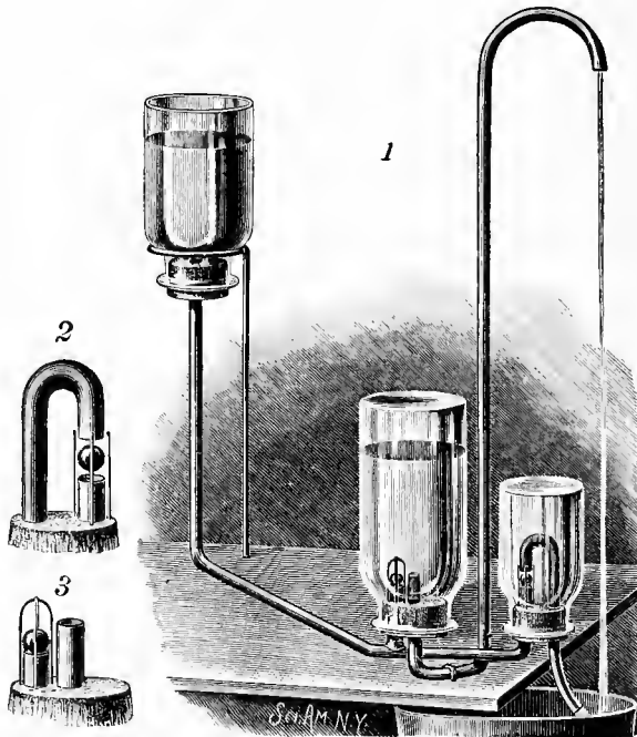
Hydraulic Ram.
