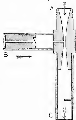
Chapman's Aspirator.
