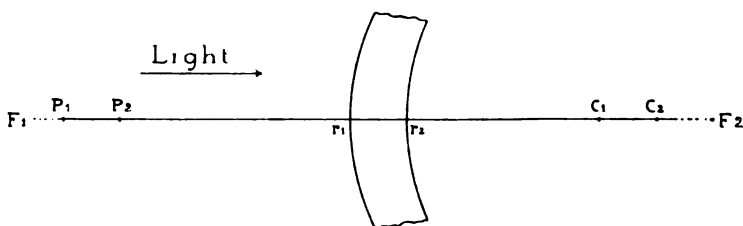
FIG. 56.—No-curvature lens.
