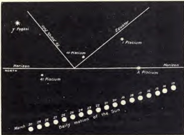
FIG. 25.—Positions of the Sun below the East horizon, near the Spring Equinox, at the rising of λ Piscium.
