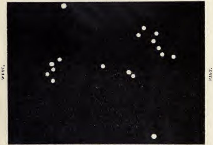
FIG. 1.—Looking north at Midnight on JANUARY 13.
