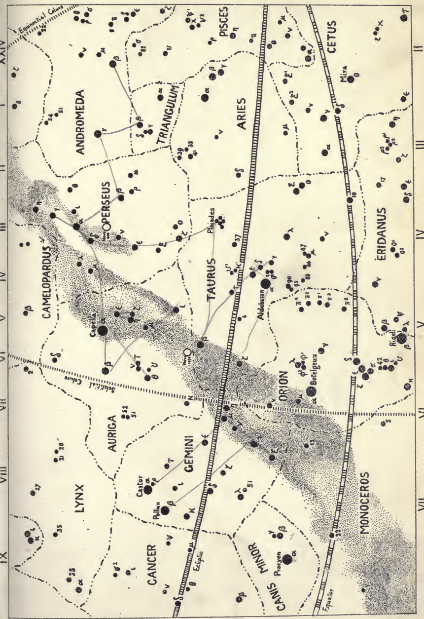
Star Map No. 10; The Region of Orion and the Bull.
