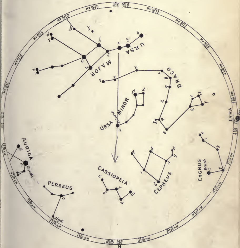
FIG. 13.—The Chief Circumpolar Stars, midnight, April 1st.
