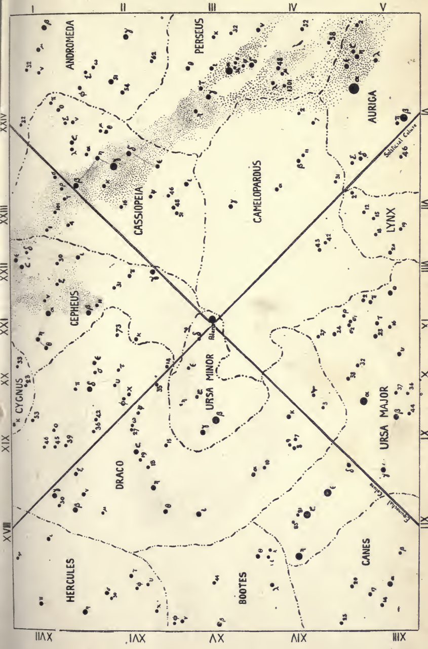
Star Map No. 1; The North Circumpolar Region.
