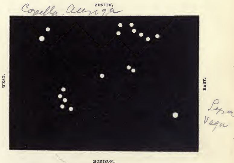
FIG. 2.—Looking north at Midnight on FEBRUARY 13.
