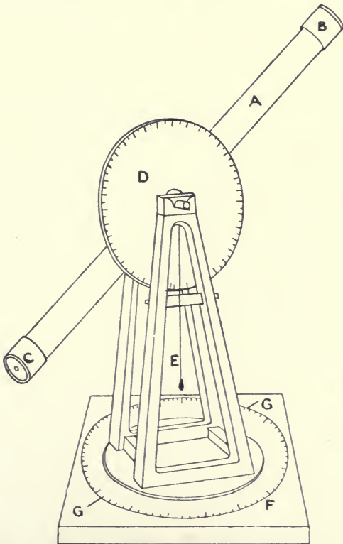
FIG. 24.—Pinhole Altazimuth for Observation of the Sun.
