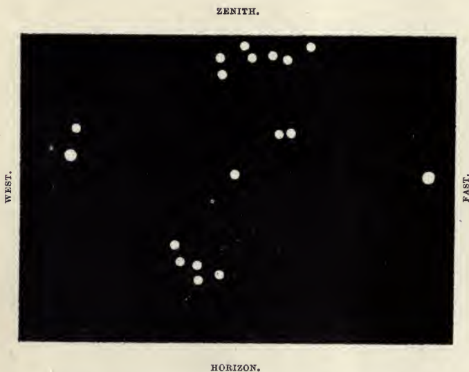
FIG. 3.—Looking north at Midnight on MARCH 15.
