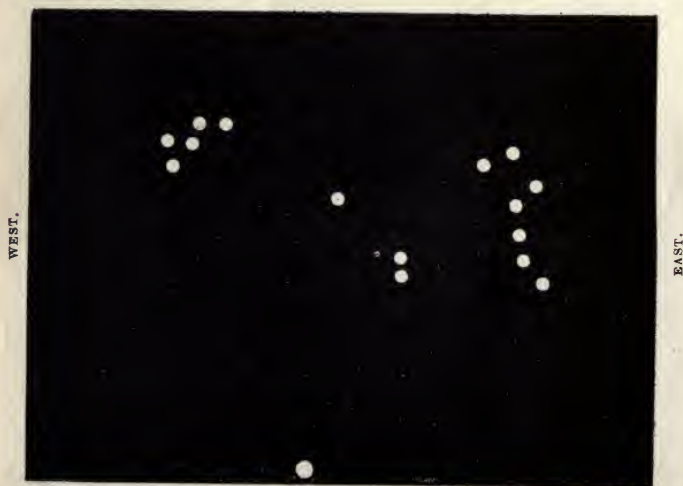
FIG. 12.—Looking north at Midnight on DECEMBER 14.
