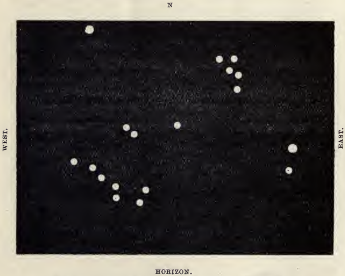
FIG. 8.—Looking north at Midnight on AUGUST 14.
