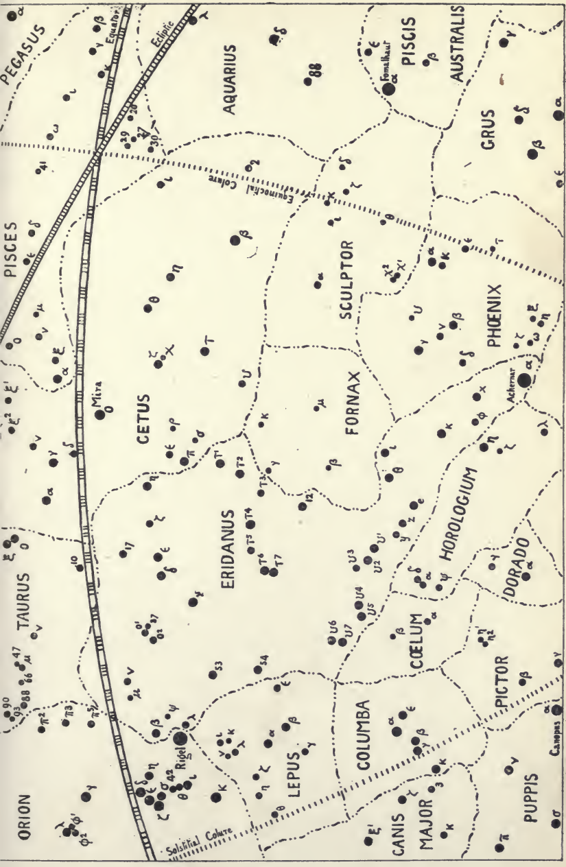
Star Map No. 9; The Region of the Sea-Monster and the Flood.
