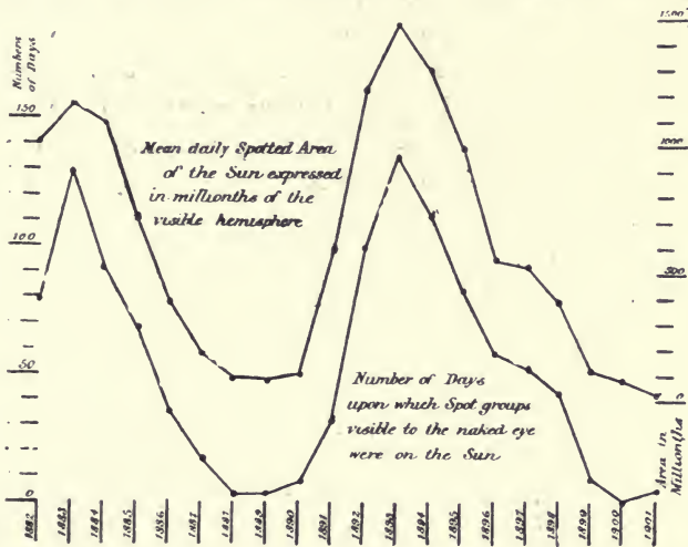
FIG. 32.—Sunspot Curves; 1882 to 1891.
