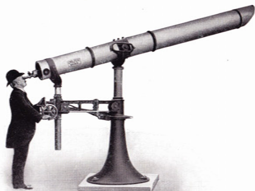
Fig. 29. 8 \frac{3}{4} inch. Observation Telescope. Magn. 70 \times , 120 \times , 200 \times . 9239 With triple revolving eyepiece. Tube length 169 inches. Codeword: Asalado .
