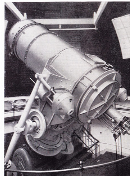
39¼ inch. Reflector of the Hamburg Observatory at Bergedorf. 9217
