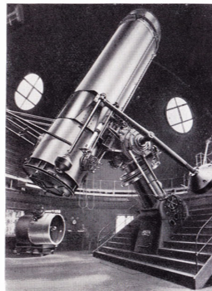
49 inch. Reflector of the Observatory at Berlin-Babelsberg. 9212
