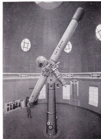
25½ inch. Refractor of Berlin-Babelsberg with Rising Floor in its lowest position. 9216
