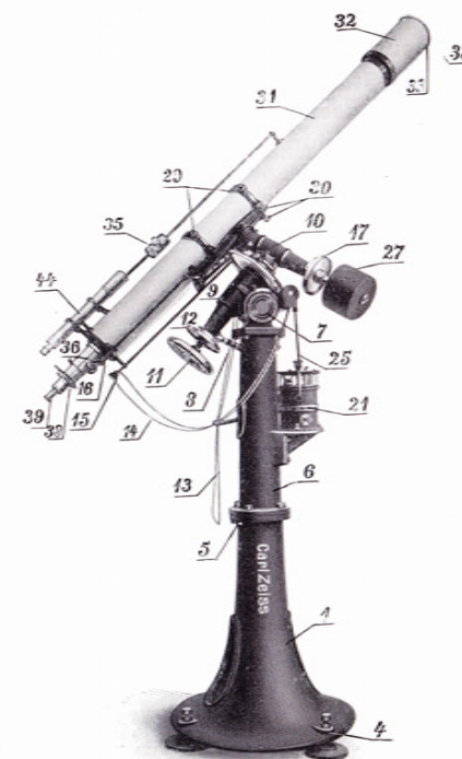
Fig. 33. Equatorial of 4 \frac{1}{4} or 5 \frac{1}{4} inch. aperture.
