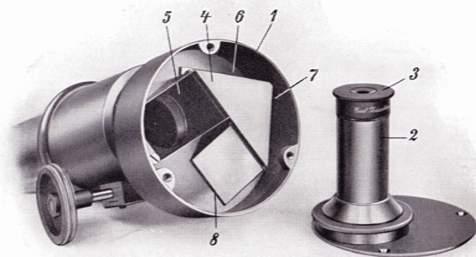
Fig. 35. Set of Erecting Prisms.
