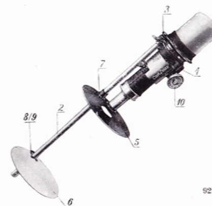
Fig. 37. Sun Projection Screen attached to the 60 mm (2 1/2 inch.) Asegur Telescope.
