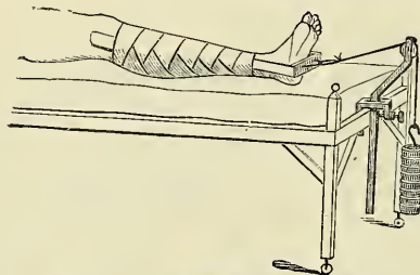
6061.* Dr. Levis' Extension Apparatus.
