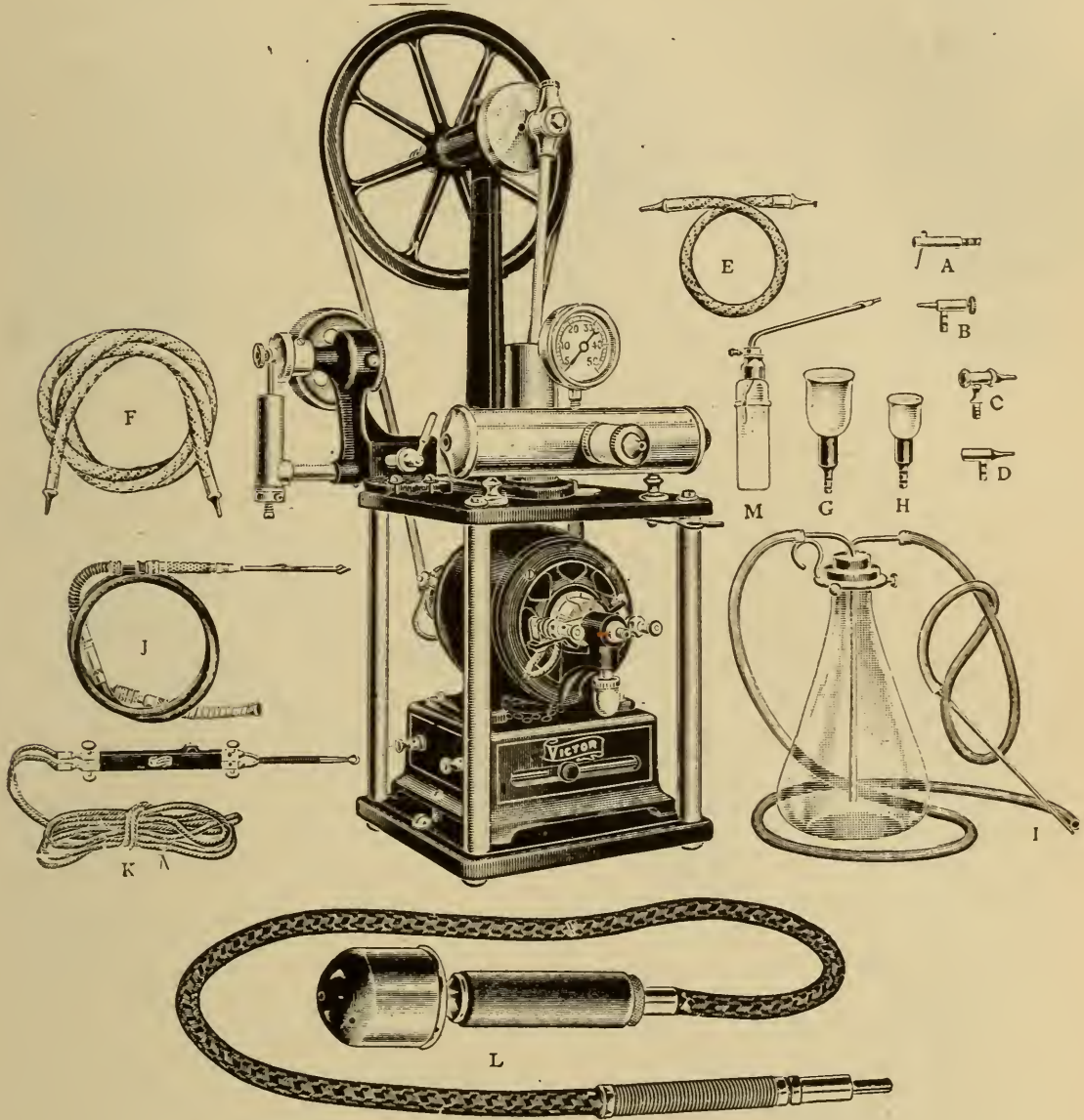
Fig. 1 (VICTOR "NO. 8" TANKLESS)
