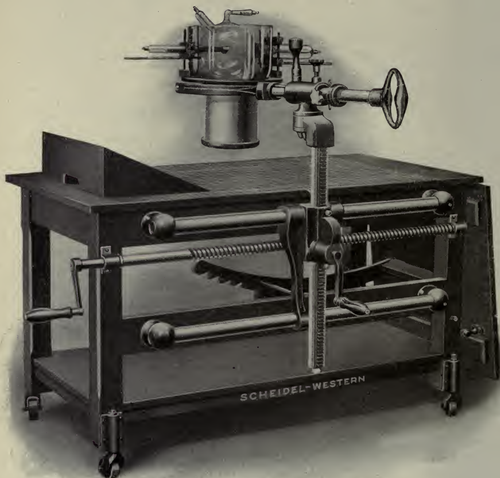
F-798. SCHEIDEL-WESTERN RADIOGRAPHIC TABLE AND COMPRESSION DIAPHRAGM.
